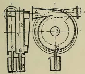
FIG. 70.—Centrifugal Deflector.
